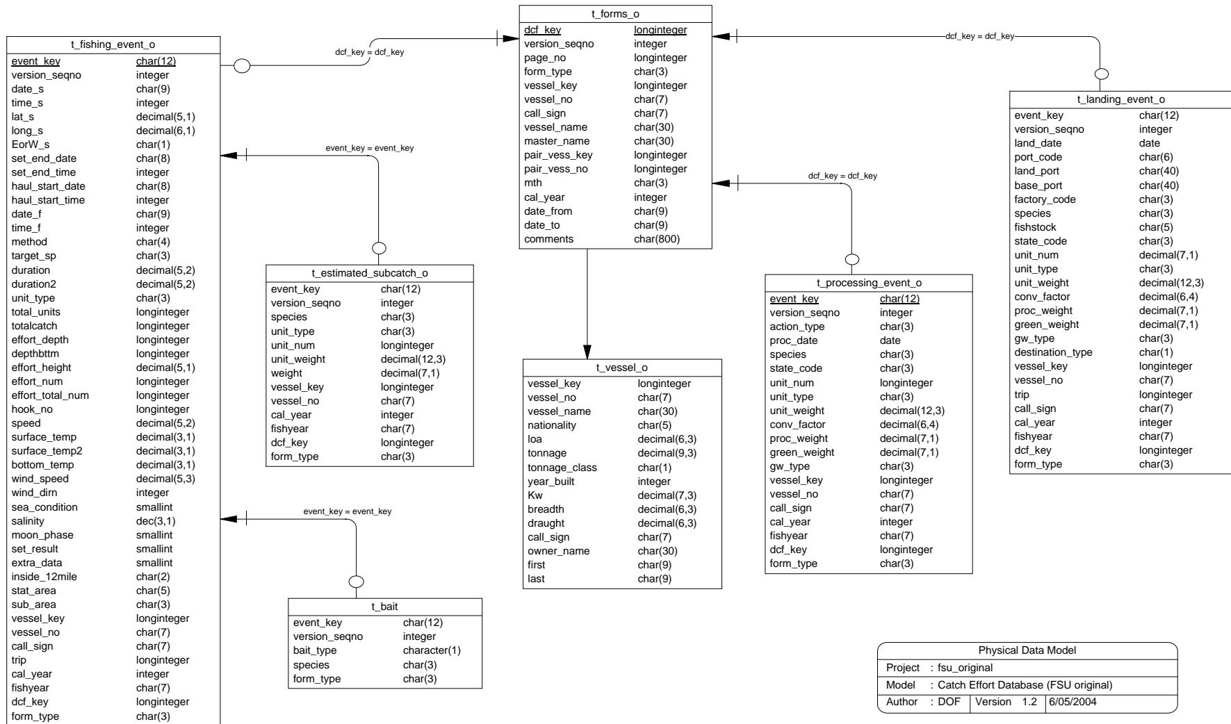
Figure 2: Entity Relationship Diagram (ERD) for the original tables in this new_fsu database
