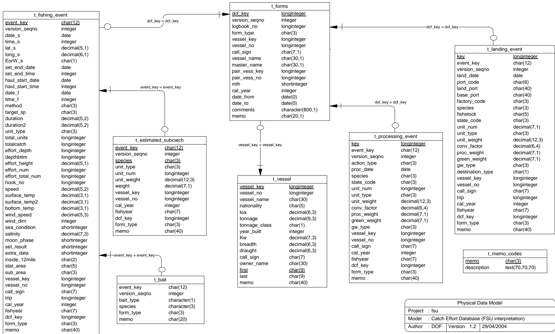
Figure 1: Entity Relationship Diagram (ERD) for this new_fsu database
